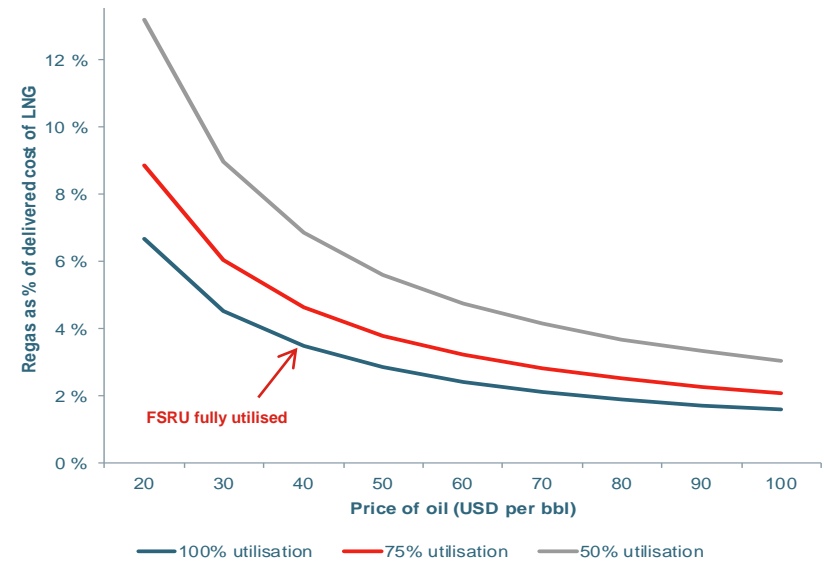
Regasification costs - FSRU
